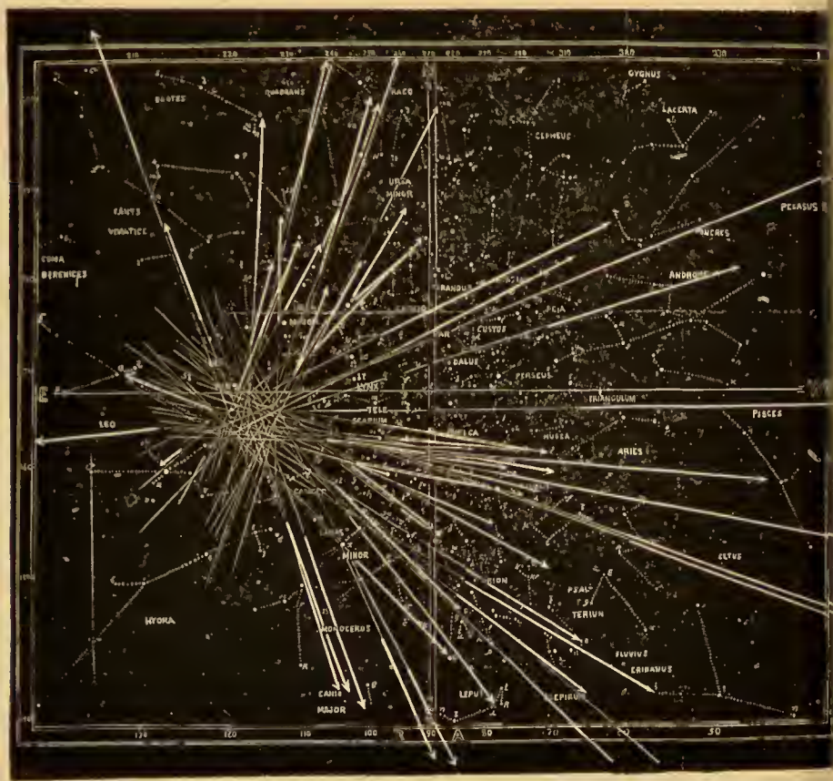
FIG. 105.—Radiant point perspective. The arrows represent a number of approximately parallel meteor-streaks foreshortened from a common vanishing-point.
